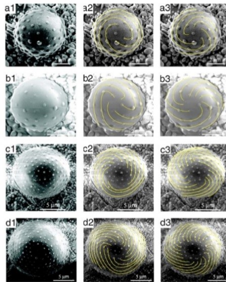
FIG. 1. Fibonacci spiral patterns in the sinister form grown on Ag-core/SiO 2 shell microstructures: (a) 3x5, (b) 5x8, (c) 8x13 and (d) 13x21.
