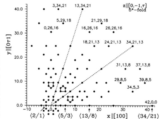
Fig. 3. — Universal pseudo-fivefold electron-diffraction pattern of the Fibonacci crystals (incident beam falls along z direction). All x -coordinates are integer: x_{rel} = h . Only about one fourth of the pattern is shown; the complete picture can be obtained by the mirror reflections: x \rightarrow -x and (or) y \rightarrow -y . The scale of the pattern are determined by the positions of the most intense edge reflections ( Q \approx 3 \text{ \AA}^{-1} ); for the different Fibonacci crystals those positions are marked by arrows. The Miller indices are shown for outer reflections only; the indices of inner reflections can be obtained from the outer ones after multiplication by factor \tau^{-i} ( i = 1, 2, 3, \dots ) and round-up to the closest integer. The innermost ten reflections are of the type \langle 200 \rangle and \langle 211 \rangle . The approximate \tau -inflation is clearly seen in the figure (pentagons with strongest distortions are marked with solid lines). Pseudo-two-fold axes are shown by dashed lines.
