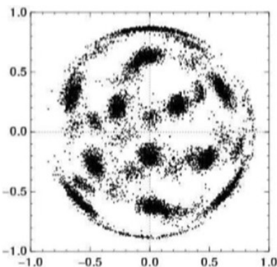
Fig. 10. Full sky map showing the optimal dodecahedral orientation for the ILC map with the kp2 mask, as for Fig. 5, centred on the North Galactic Pole
