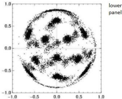
Fig. 5. Full sky map showing the optimal orientation of dodecahedral face centres based on 100,000 steps in 10 MCMC chains, using the ILC map and either the kp2 mask (upper panel) or no mask (lower panel), showing face centres for which P > 0.5 (see Eq. (25)). The projection is a Lambert azimuthal equal area projection (Lambert 1772) of the full sky, centred on the North Galactic Pole (NGP). The 0^\circ meridian is the positive vertical axis and galactic longitude increases clockwise. These face centres are derived from the MCMC chains without any constraint on the twist phase \phi .
