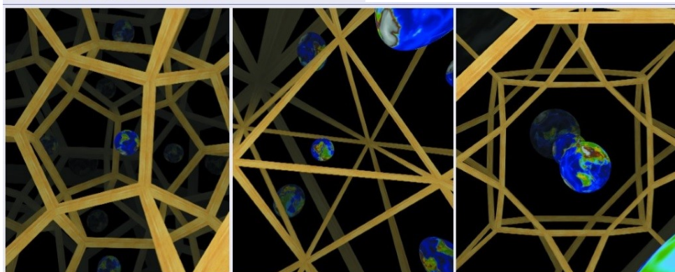
The Poincaré dodecahedral space (left) can be described as the interior of a "sphere" made from 12 slightly curved pentagons. However, there is one big difference between this shape and a football because when one goes out from a pentagonal face, one immediately comes back inside the ball from the opposite face after a 36° rotation. Such a multiply connected space can therefore generate multiple images of the same object, such as a planet or a photon. Other such well-proportioned, spherical spaces that fit the WMAP data are the tetrahedron (middle) and octahedron (right).
