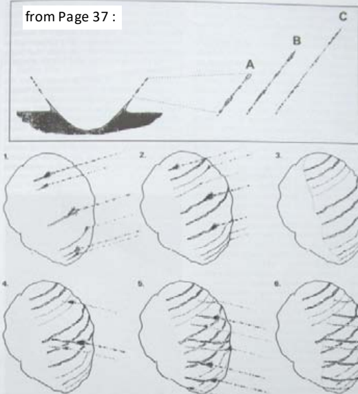
Fig. 17. Diagrams illustrating the formation of Phobos' grooves by the impact of ejecta from large impacts on Mars, from Murray et al. (1994). The top diagram shows a section through a large impact event on Mars, early in crater excavation. Highly shocked and melted material from both the impactor and the impacted surface is ejected at velocities of several km s -1 in a cone whose apex is the crater centre. The velocity of ejecta rapidly decays with time, so the leading part of each individual ejected jet of melt will steadily draw away from the following end and cause it to be stretched out into a progressively longer string of apices, as at A, B and C. The lower series of diagrams (1-6) shows the situation at Phobos. (1) and (2) Show radial (effectively parallel at the distance of Phobos) ejecta strings from the same impact on Mars arriving at Phobos, where Phobos' motion in its orbit (towards the lower right of the observer) causes long chains of secondary impact craters to form on its surface. (3) Shows the situation after the shower of debris has passed: nearly one half of Phobos is crossed with parallel grooves composed of contiguous secondary impact craters with raised rims. (4) and (5) Show the situation at a later time, when a different large impact on Mars results in the arrival of a second shower of ejecta, causing new parallel grooves to form at a different orientation from the earlier set. (6) Shows the final situation, with two families of parallel grooves crossing each other, each family covering only one half of Phobos.
