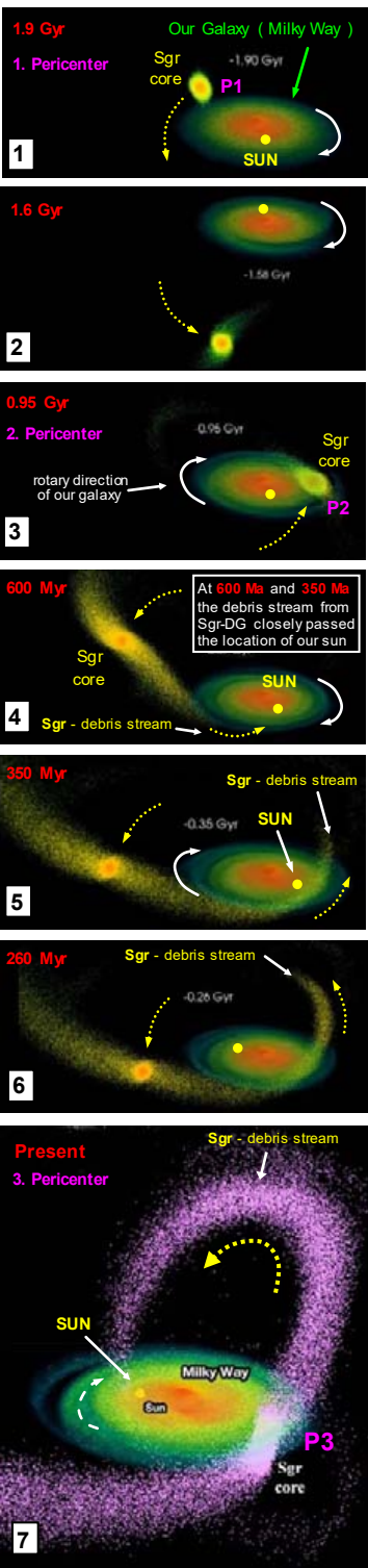
Figure 1 - Image sequence showing the last three pericenter events in quick-motion ( images 1 to 7 & 1 to 4).
