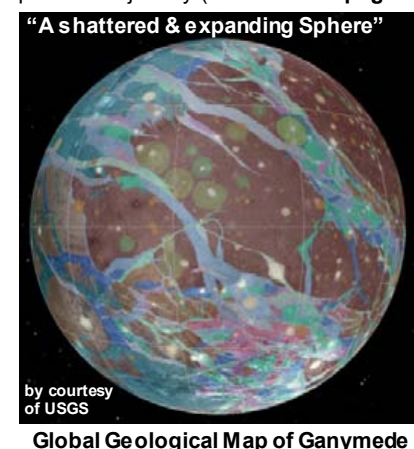
Global Geological Map of Ganymede
