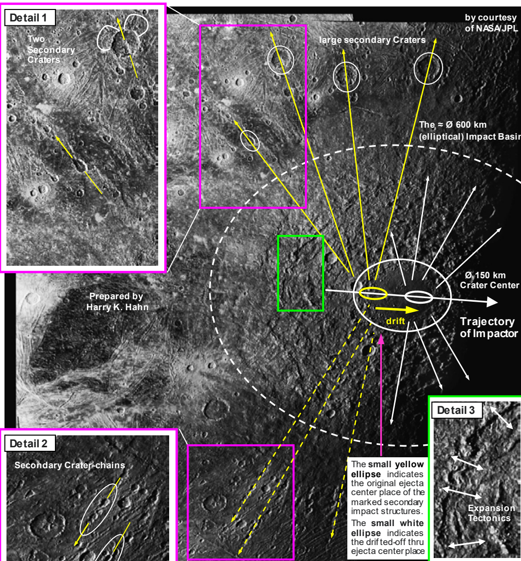
Gilgamesh Impact Basin on Ganymede : The \varnothing 600\text{ km} (elliptical) impact Basin ( w white dashed line ) and the inner \varnothing 150\text{ km} elliptical crater center indicate an \approx 10^\circ shallow (oblique) Impact. Secondary crater chains & secondary impacts and expansion tectonics indicate that the crater drifted away from the original impact site ( w white arrow )
