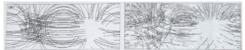
(e) (Lower left) Predicted secondary crater chain orientations from impacts at 12 different latitudes on Mars, chosen to match those seen on Phobos. Note the resemblance between this model and the map of grooves at the bottom. The model is simplified as a spherical Phobos, so does not fit the real situation as well as if it were modelled as a triaxial ellipsoid; nevertheless, the resemblance between theory and model illustrated in (e) is strong. (f) (Bottom right) Map of Phobos' grooves from HRSC images.
