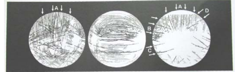
Fig. 7. (Top) Orthographic projections of groove positions on Phobos centred on (left) the leading apex (0° latitude, 90° longitude), (centre) the sub-Mars point and (right) the trailing apex. Note that grooves appear straight and in groups of parallel families when viewed from the leading and trailing apex (left and right). Four prominent families were named by Thomas et al. (1979); family A (the most prominent and numerous), B and D are marked. Also, note that all grooves become parallel along the sub-Mars meridian. from Page 28 :
