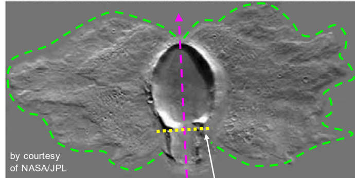
Example Mars Impact with Butterfly Ejecta Distribution Credit: NASA / JPL / ASU / mosaic by Emily Lakdawalla Owing to the atmospheric drag, a string of fragmented impactors would differentiate during decent, with the larger bodies tending to travel further than smaller ones. We call special attention to the work of Schultz and Stöckle ( Lost Impacts ), which explains how shallow angle of incidence (oblique) impacts generate "impact" structures that are significantly different from the classic, better understood, crater planforms. We proposed the Saginaw impacts to have been at an angle of less than 5 degrees - nearly tangential. The craters generated would manifest
