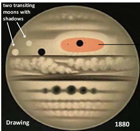
Drawing from E. Trouvelot 1880; A photo from 1879 of Jupiter from Anne Clerk's Book \rightarrow see : Weblink
