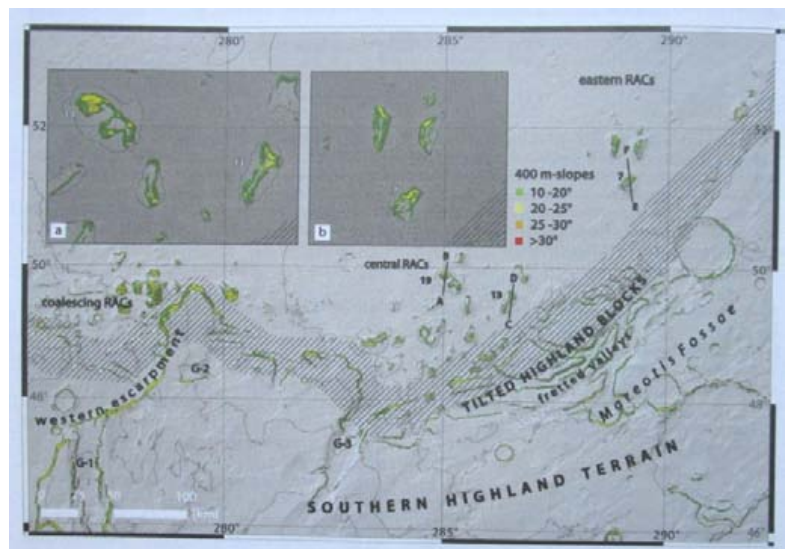
Fig. 5. Map in a hillshade-relief representation with superimposed slope data of remnant massifs and debris aprons. Slope data have been derived from 400 x 400 m digital terrain model data to avoid low-frequency noise. Locations of topographical profiles are located. North is up in all images.
