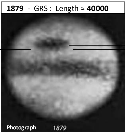
Drawing from E. Trouvelot 1880; A photo from 1879 of Jupiter from Anne Clerk's Book \rightarrow see : Weblink
