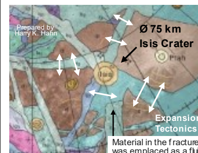
Material in the fractures was emplaced as a fluid (water, slush or solid ice warm enough to flow).
